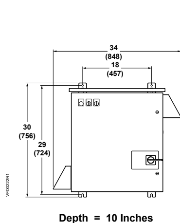
Enclosure Frame B
